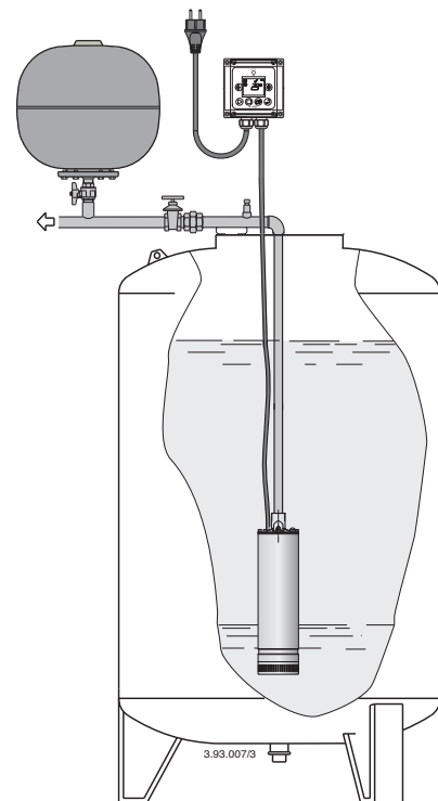
Installation examples
