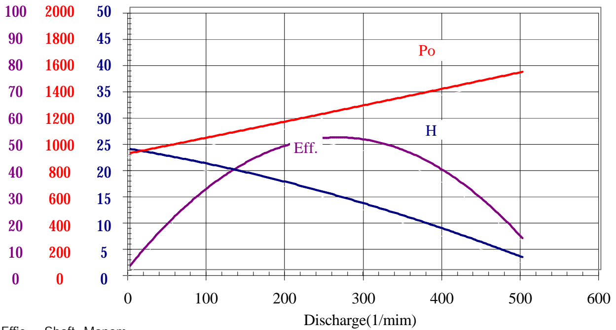
PUMP Performance Curve
